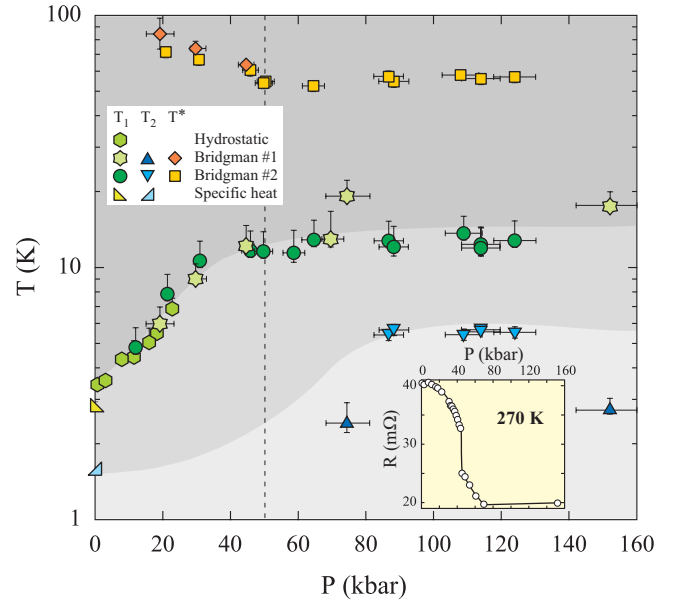
FIG. 4. (Color online) Temperature versus pressure phase diagram for \text{CeTe}_3 (note the logarithmic temperature scale). T^* characteristic temperature associated with the “humplike” feature in \rho(T) , possible origins of which are discussed in the text; T_1 magnetic ordering temperature; T_2 ordering temperature (probably magnetic). The vertical dashed line separates the T - P phase diagram into two regions in which T^* , T_1 , and T_2 all have distinctly different pressure dependencies. We grouped in a single low-temperature magnetic phase the critical temperatures T_2 obtained from measurements of the electrical resistivity under pressure and specific heat at ambient pressure, although they might have different origins. Inset: room-temperature evolution of the electrical resistance as the pressure was increased. The abrupt jump at 45 kbar may be due to a structural phase transition.
