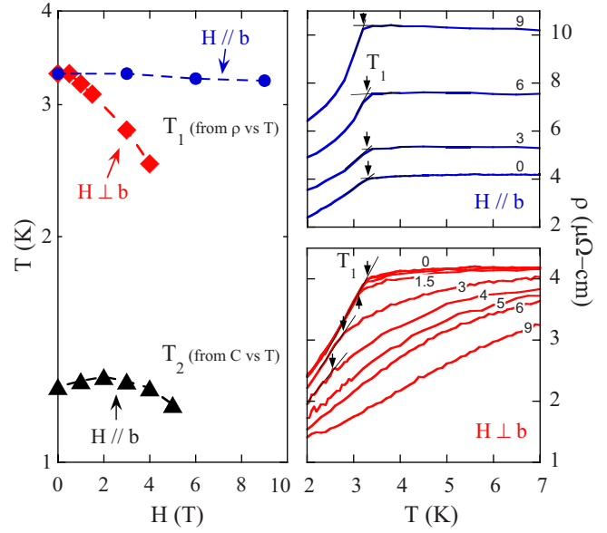
FIG. 3. (Color online) Left: field dependence of the magnetic ordering temperatures T_{1,\rho} and T_{2,C} of \text{CeTe}_3 for magnetic fields applied perpendicular and parallel to the b axis. A logarithmic temperature scale was chosen to emphasize the curvature of T_2 vs H . Right: temperature dependence of the electrical resistivity near T_1 for magnetic fields applied parallel (upper right: 0, 3, 6, and 9 T) and perpendicular (lower right: 0, 0.5, 1, 1.5, 3, 4, 5, 6, and 9 T) to the b axis of the crystals. The arrows mark the position of T_1 . The numbers on each curve denote the value of the applied magnetic field in tesla. For the lower-right panel, arrows and numbers for fields of 0.5 and 1 T are not displayed for better clarity.
